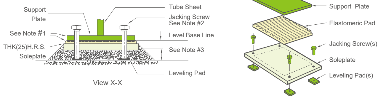
Rubber Isolation
